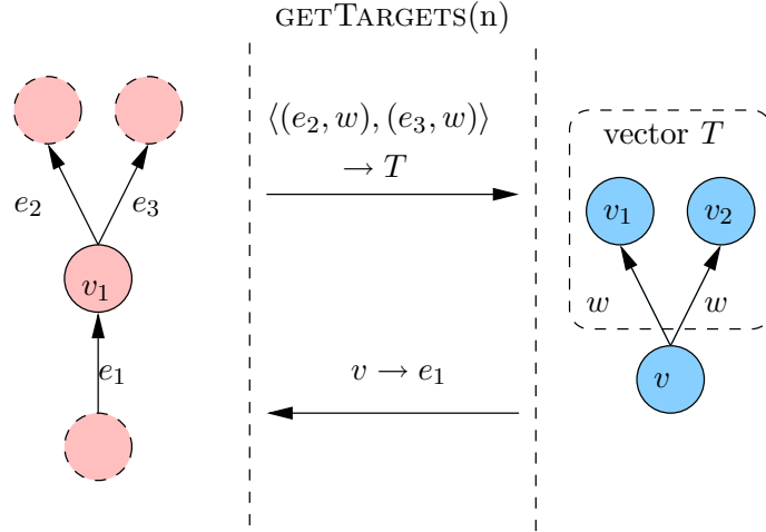
Figure 6: The GETTARGETS() method interacting with both, the node-based and the edge-based graphs.
