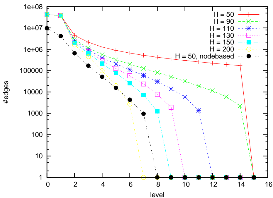
Figure 8: Different neighbourhood sizes H have a significant impact on the number of levels. The experiments were conducted using an offline-converted version of the graph representing the road network of Germany. Turn-costs were included. For comparison, the diagram contains results for the node-based graph as well, where experiments have shown a neighbourhood size of 50 to be a good choice.
