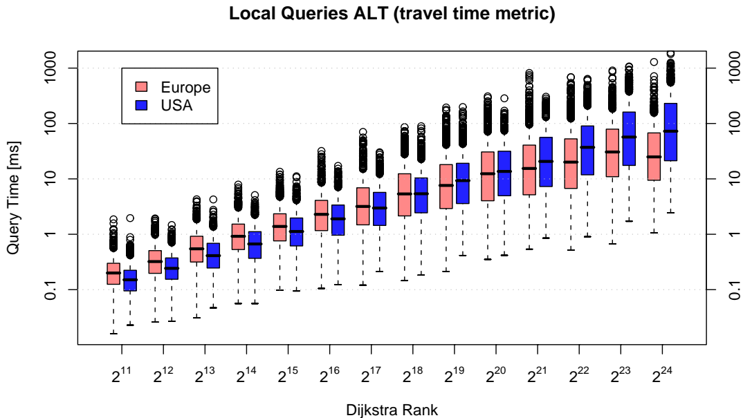
Fig. 5. Comparison of the query times using the Dijkstra rank methodology on the road networks of Europe and the US. The landmarks are chosen from the level-3 core using maxCover. The results are represented as box-and-whisker plot [19]: each box spreads from the lower to the upper quartile and contains the median, the whiskers extend to the minimum and maximum value omitting outliers, which are plotted individually.
