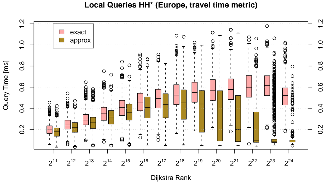
Fig. 6. Comparison of the query times of the exact and the approximate HH* search using the Dijkstra rank methodology.
