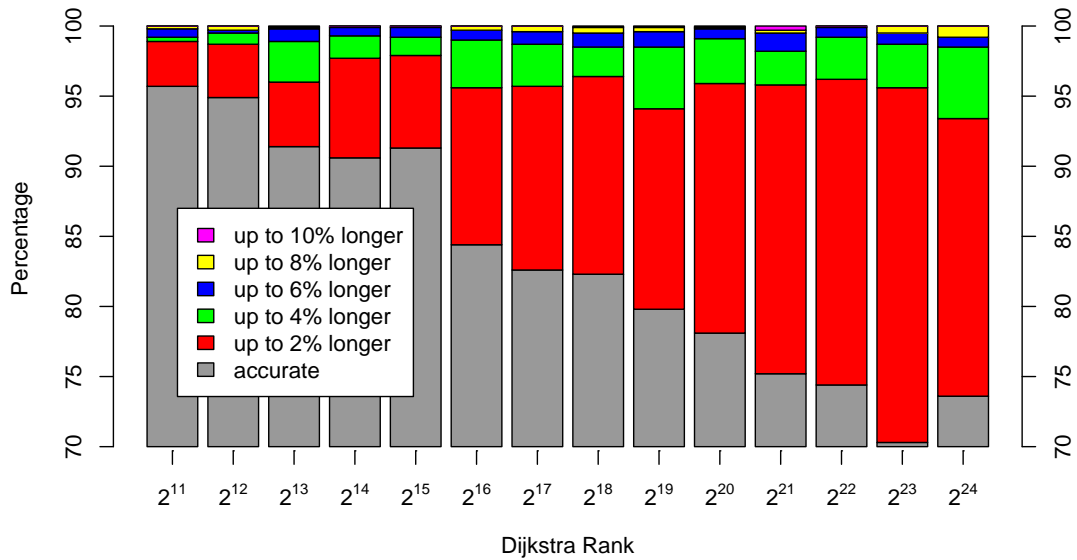
Fig. 16. Actual distribution of the approximation error for a random sample, grouped by Dijkstra rank. Note that, in order to increase readability, the y-axis starts at 70%, i.e., at least 70% of all queries returned an accurate result.
