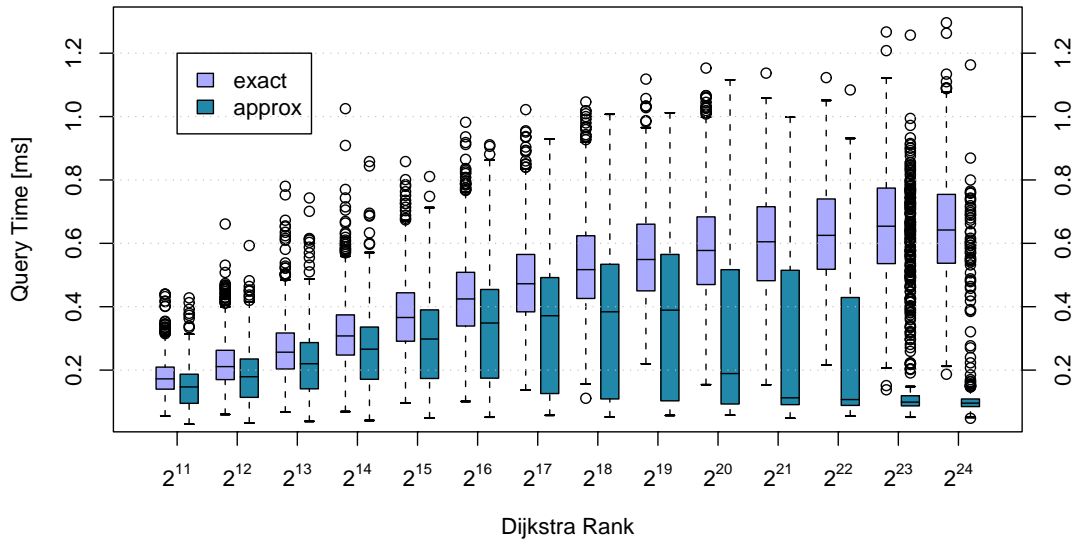
Fig. 15. Comparison of the query times of the exact and the approximate HH* search.
